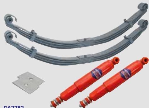
DA2782 Parabolic Spring Kit - Rear Series - LWB 2 x Parabolic spring - 4-leaf 2 x Long travel Cellular Dynamic shock absorbers 2 x Angle correction wedges
