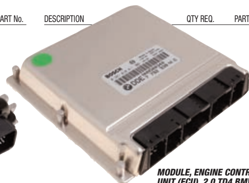
MODULE, ENGINE CONTROL UNIT (ECU), 2.5 KV6 - NNN000180
