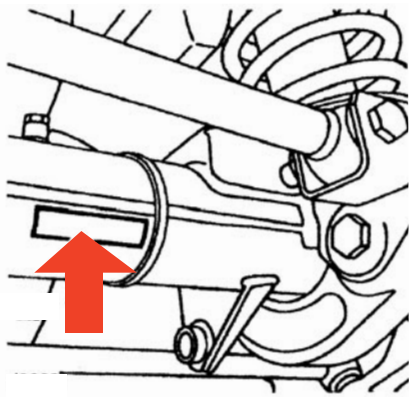
THE FRONT AXLE SERIAL NUMBER IS STAMPED ON THE FRONT OF THE LH AXLE TUBE, INBOARD OF RADIUS ARM MOUNTING BRACKET.
