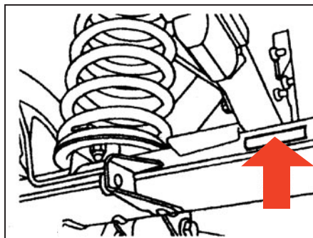
THE REAR AXLE SERIAL NUMBER IS STAMPED ON THE REAR OF THE LH AXLE TUBE, INBOARD OF SPRING MOUNTING.
