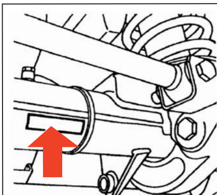
THE FRONT AXLE SERIAL NUMBER IS STAMPED ON THE FRONT OF THE LH AXLE TUBE, INBOARD OF RADIUS ARM MOUNTING BRACKET.
