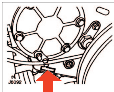
THE TRANSFER GEARBOX LT230 SERIAL NUMBER IS STAMPED ON THE GEARBOX CASING BELOW THE MAINSHAFT REAR BEARING HOUSING.
